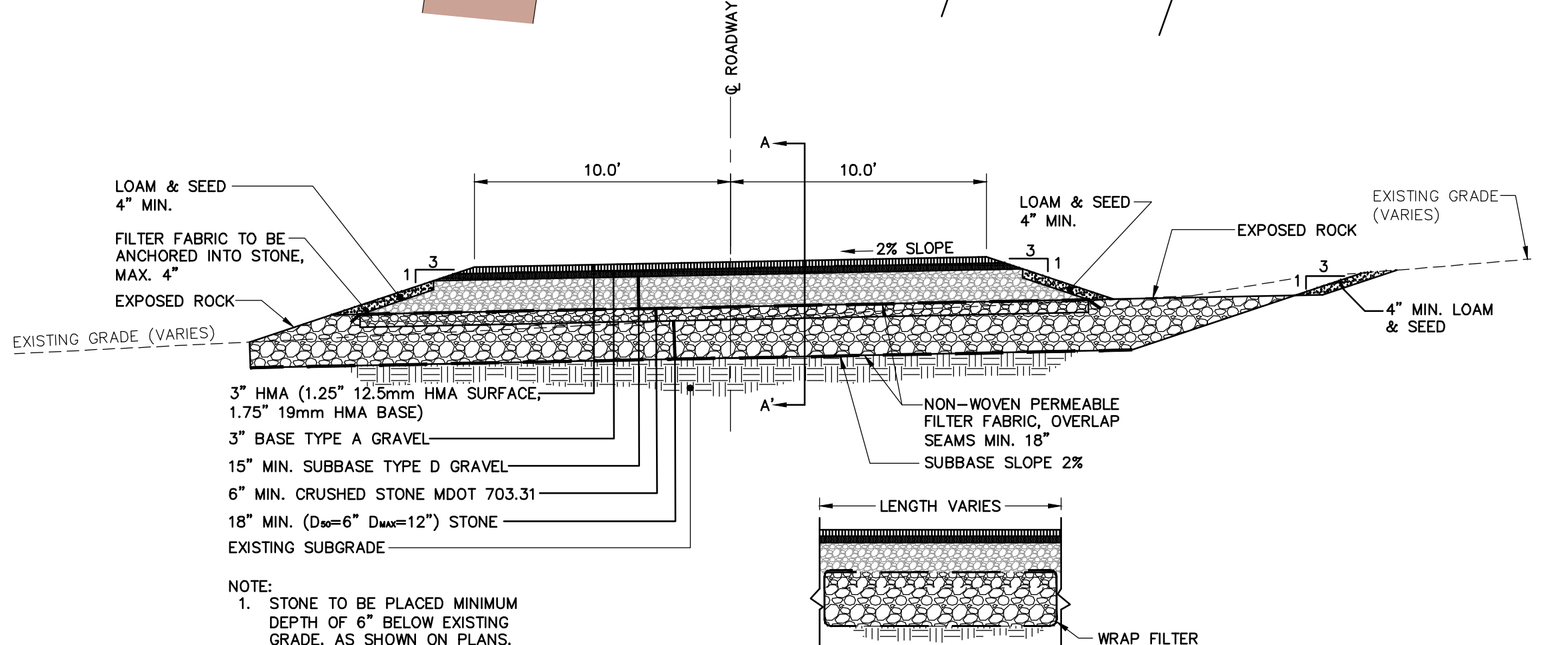
ROCK SANDWICH #2 SCALE: 1"=5'
