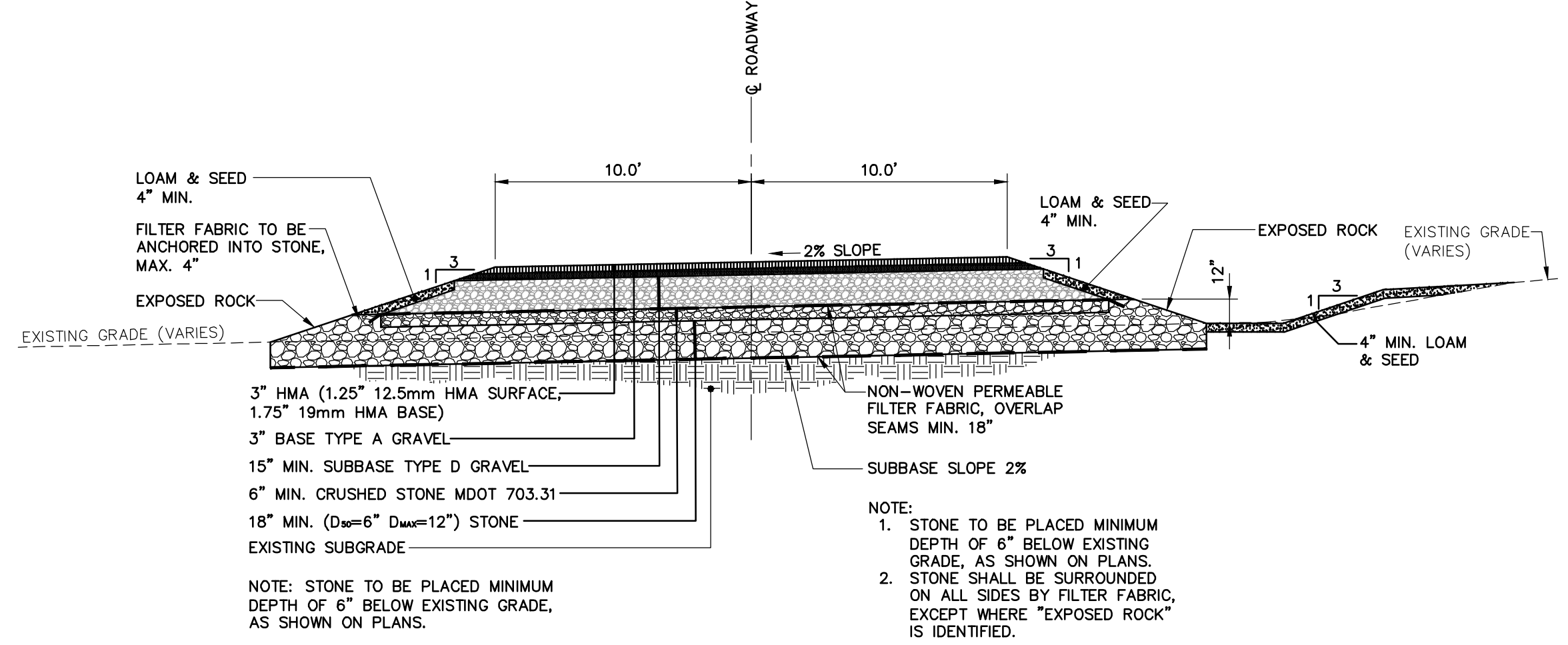
ROCK SANDWICH #1 SCALE: 1"=5'
